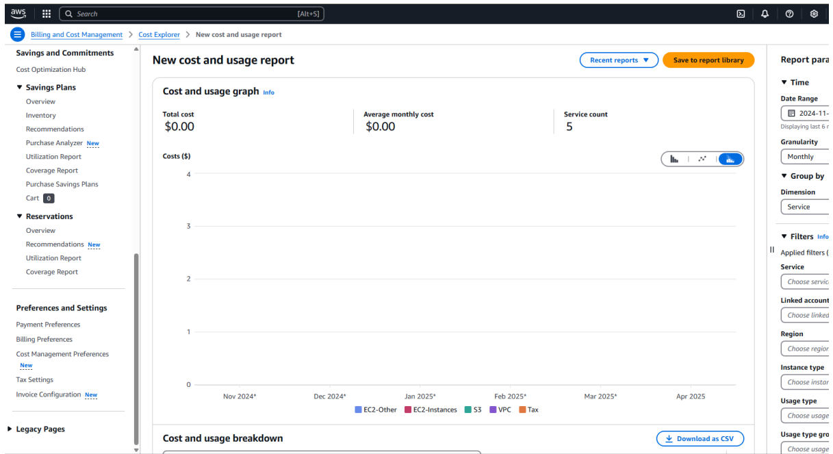
Fig 4.1 Billing Dashboard
