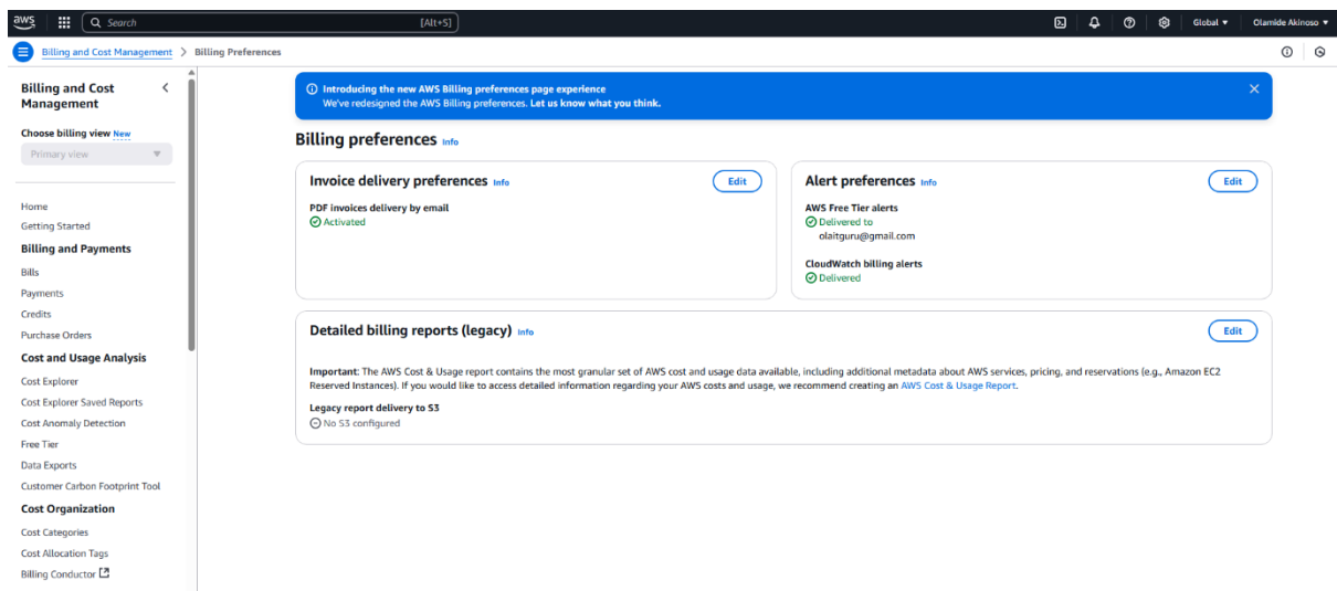
Fig 4.2 Enabling Alerts
